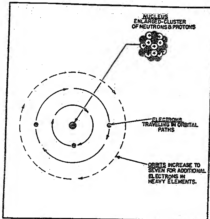
Figure 1—Diagram of an Atom.
